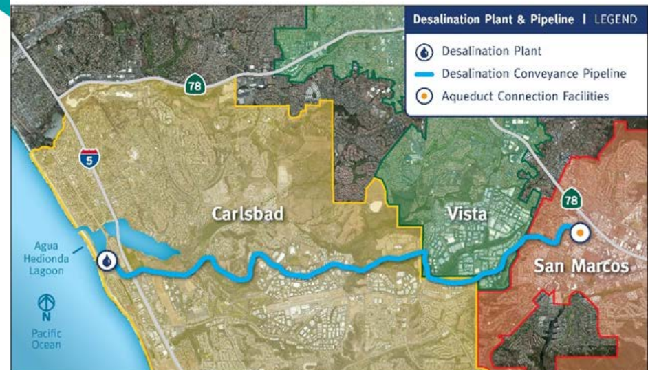
The Carlsbad Desalination Pipeline Route
